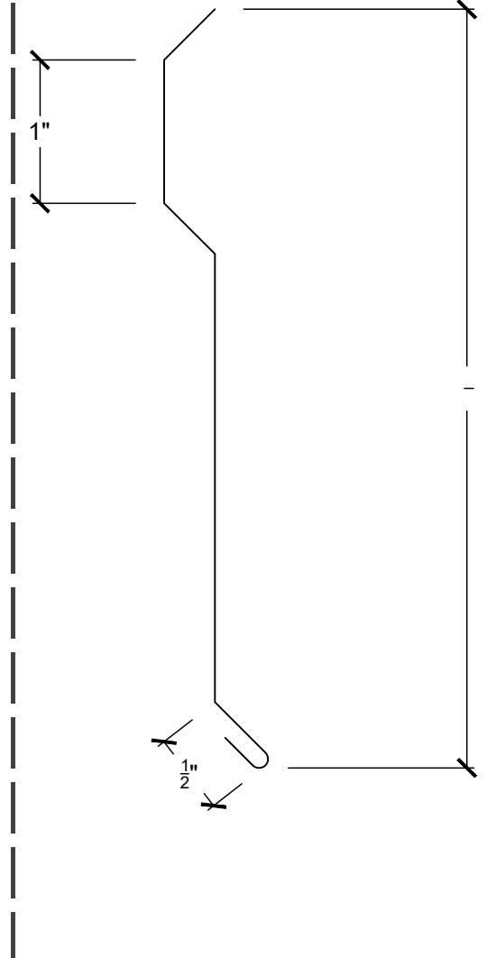
SURFACE MOUNTED FLASHING (TYP. DETAIL)
