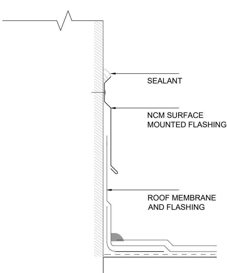
SURFACE MOUNTED FLASHING (TYP. DETAIL)
